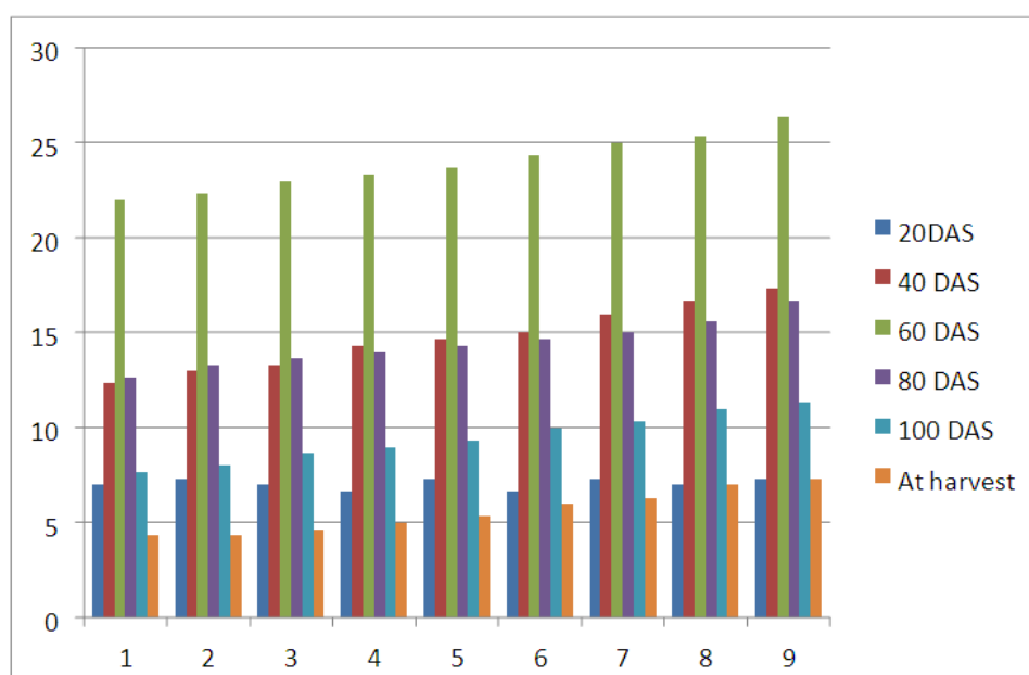
Fig. 2. Effect of Nitrogen and Sulphur on Number of nodules of lentil at different day intervals
