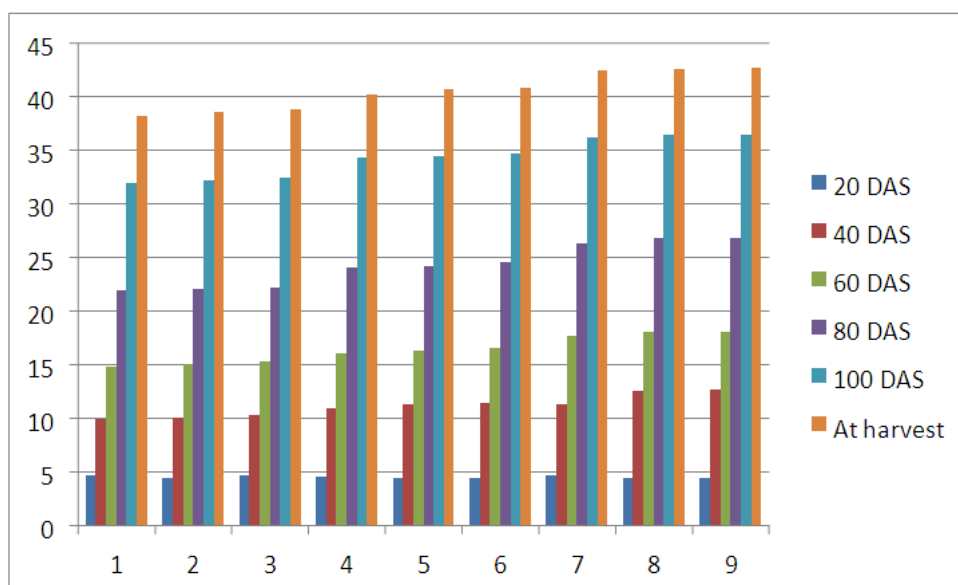
Fig. 1. Effect of Nitrogen and Sulphur on Plant height of lentil at different day interval
