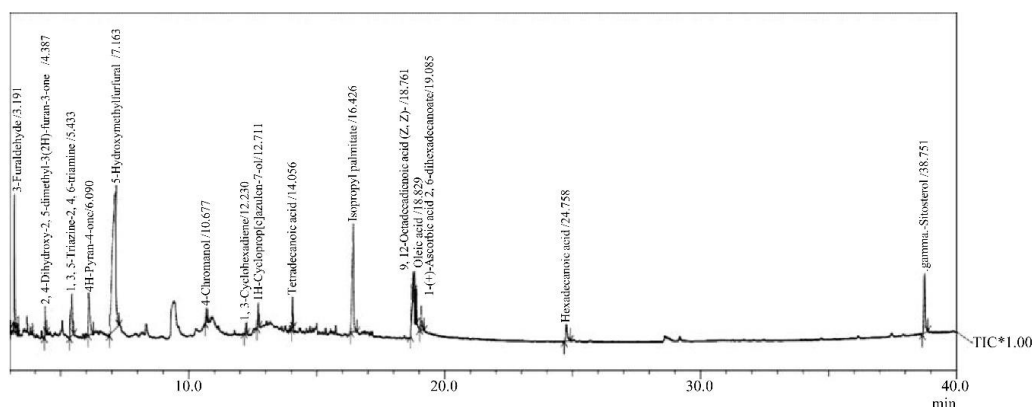
Fig. 4. GC-MS chromatogram of compounds identified in Syzygium cumini seed ethanol extract
