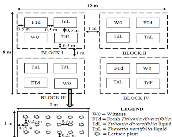
Fig. 3. Experimental device
