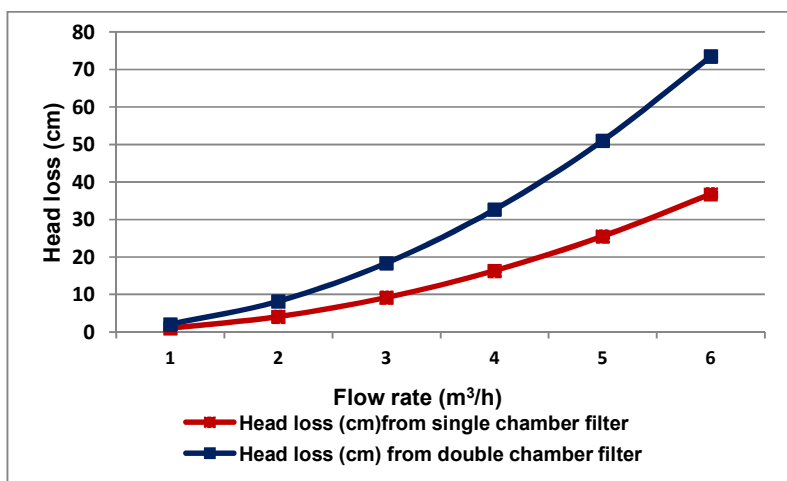
Fig. 8. Head loss vs flow rate
