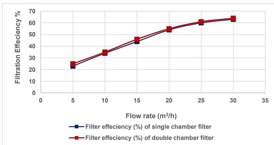
Fig. 9. Filtration efficiency vs flow rate
