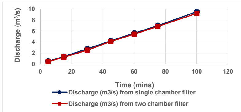
Fig. 6. Discharge vs time
