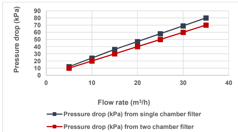
Fig. 7. Flow rate vs pressure drop
