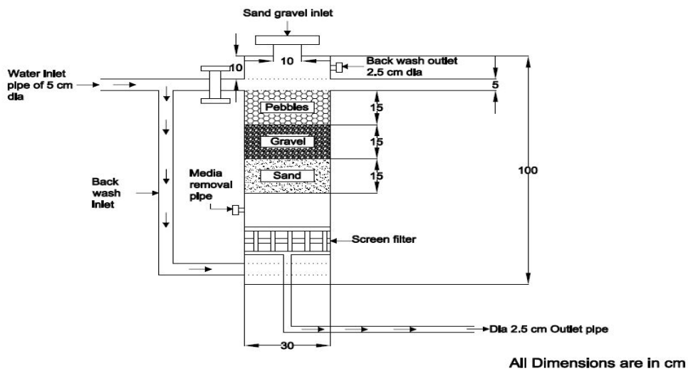
Fig. 3. Design drawing of single chamber low cost sand filter
