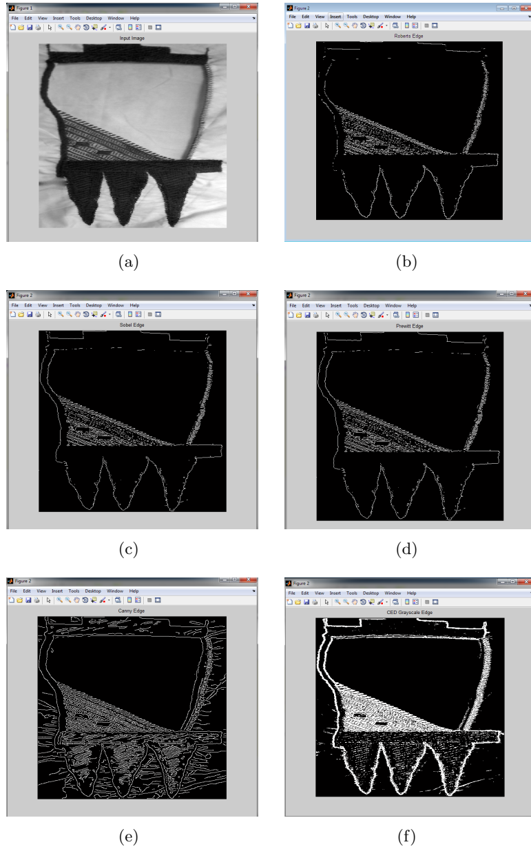
Figure 5: (a) Alábe Méta Test image (grayscale) (b) Roberts Algorithm (c) Sobel Algorithm (d) Prewitt Algorithm (e) Canny Algorithm (f) CED Algorithm
