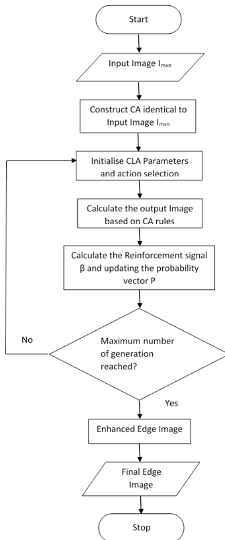
Figure 3: Cellular Edge Detection Algorithm
