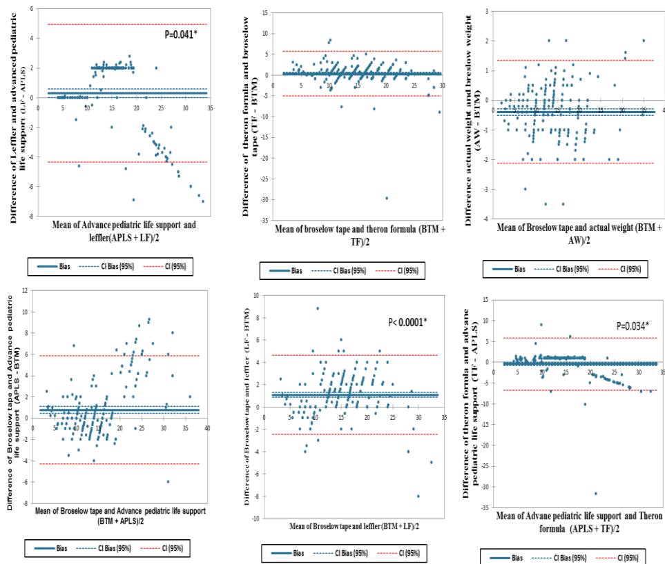
Fig. 2. Bland and Altman Plot (BTM and different weight formulas)
