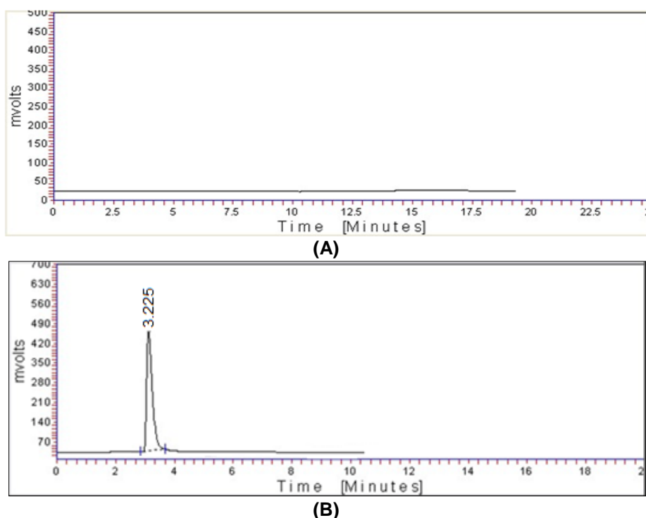
Fig. 2. Chromatograms of (A) Blank mobile phase (B) lumefantrine (15 µg/ml) as reference substances
