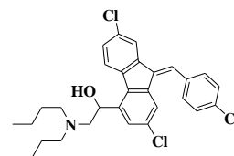
Fig. 1. Chemical structure of lumefantrine
